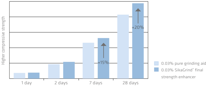
Final strength enhancement with SikaGrind® at increased production
