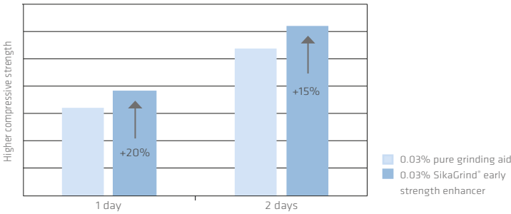
Strength enhancement with SikaGrind® due to optimized particle size distribution at constant production
