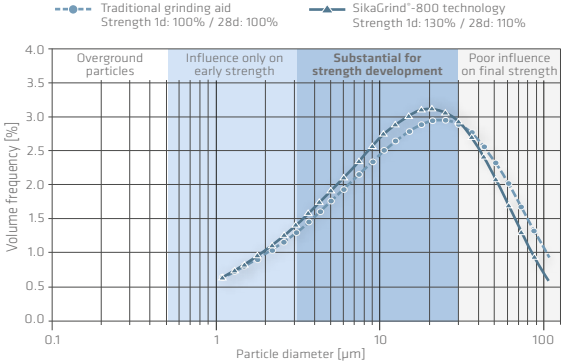
Early strength enhancement with SikaGrind® at increased production
