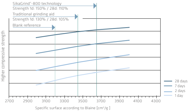
Strength enhancement with SikaGrind® due to increased fineness at constant production
