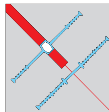
Sika Waterbar® D 320/5 DW
