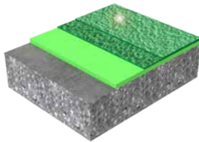
Sikafloor® PurCem HB-22 Gloss Layer thickness: 3 – 8 mm
