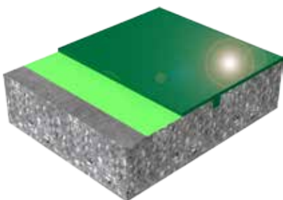
Sikafloor® PurCem HS-21 Gloss Layer thickness: 3 – 6 mm
