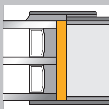
Burglary protection Sikasil® WT-480
