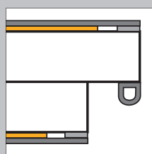
Frame and cover bonding Sikaflex®-221/-553, Sikasil® SG-500/SG-20
