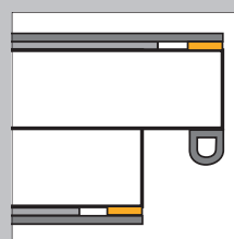
Mounting aid Sika® Glazing Tape Prefix
