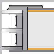
Sandwich Panel bonding SikaForce®-7710 L35
