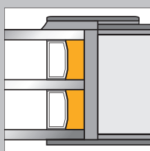
IG secondary sealing SikaGlaze® IG-25 HM plus
