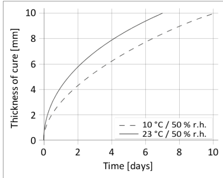
Diagram 1: Curing speed Sikaflex®-271
