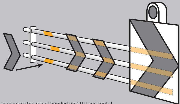
Powder coated panel bonded on GRP and metal posts with Sikaflex®-552 AT . For faster curing, Sikaflex®-953 can be used. For UV-resistant or primer-free applications, Sikasil® AS-70 or the fast cure Sikasil® AS-785 are advised.
