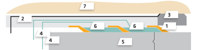
1 Wire brush | 2 Tailskin | 3 Backfill | 4 Grease lines | 5 Concrete segment | 6 Sika® Stabilizer | 7 Ground
