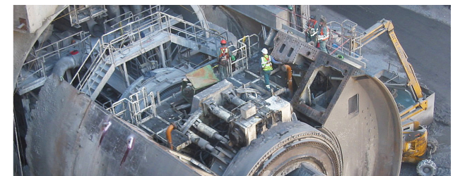
1 Sika® Stabilizer-2001 TBM | 2 Seals
