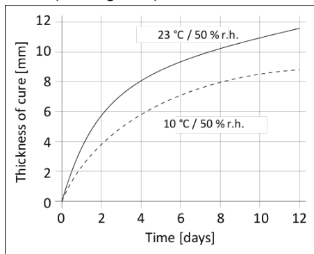
Diagram 1: Curing speed of Sikaflex® Fix
