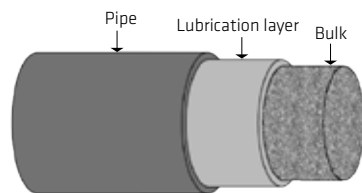
Fig. 5.8: Simplified sketch of the pumped shotcrete flow according to Kaplan et. al. 9
