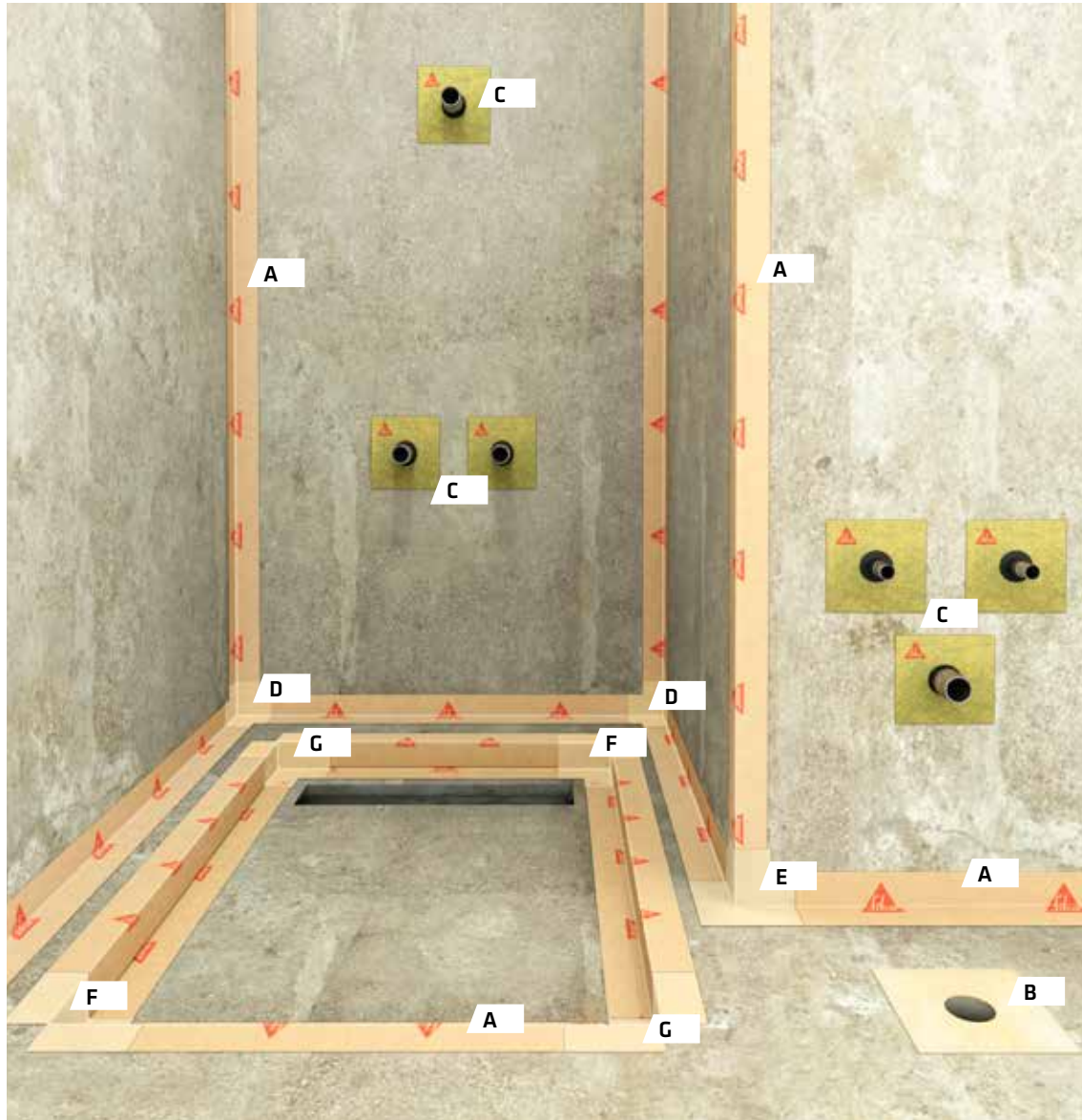
Sika® SealTape F and accessories for a watertight application.
