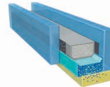
In windows with rebate bonding and glass edge bonding the IG secondary sealant is in direct contact with the window adhesive. Therefore, the adhesive must be compatible with the edge sealant. Sika's sealants and adhesive systems are tested and approved to avoid incompatibility. More information about compatibility of our systems can be found on ses.sika.com .
